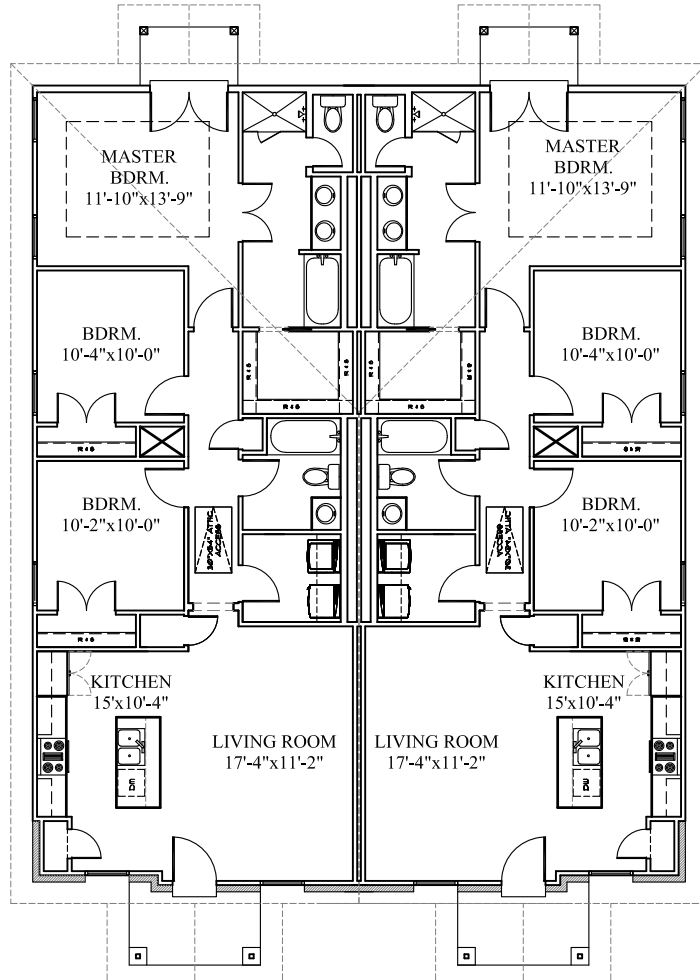
FLOOR PLAN
