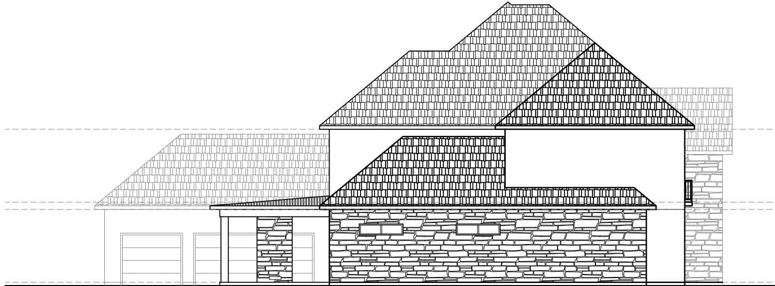
LEFT ELEVATION
