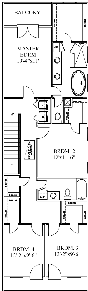
SECOND FLOOR
